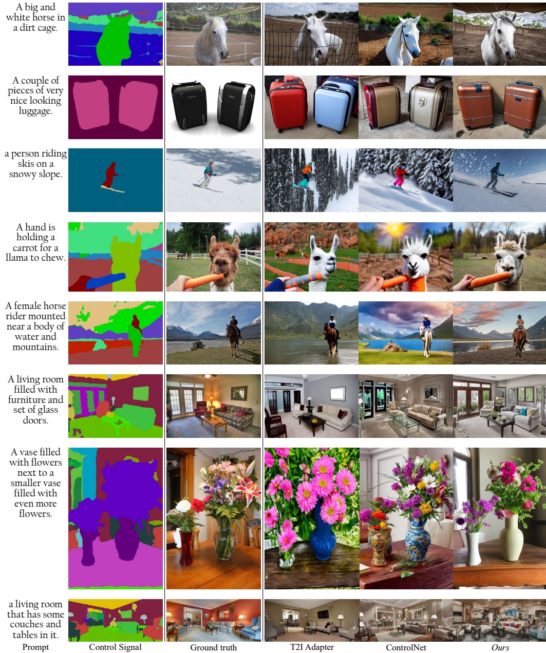
Figure 14: Additional results for Single Modality Control: Segmentation Map
