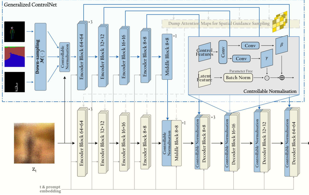
Figure 3: The network architecture of Generalized ControlNet (gControlNet) with Controllable Normalisation (ControlNorm). The parameters indicated by the yellow sections are sourced from the pre-trained model and stay constant, while only those in the blue sections are updated during training, with the gradient back-propagated along the blue arrows.
