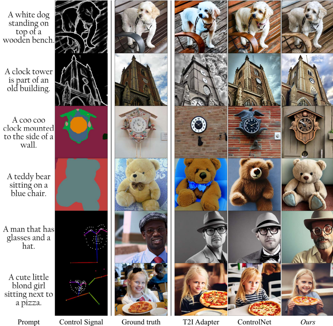
Figure 5: Qualitative comparison of Uni-Modality on the COCO validation set.
