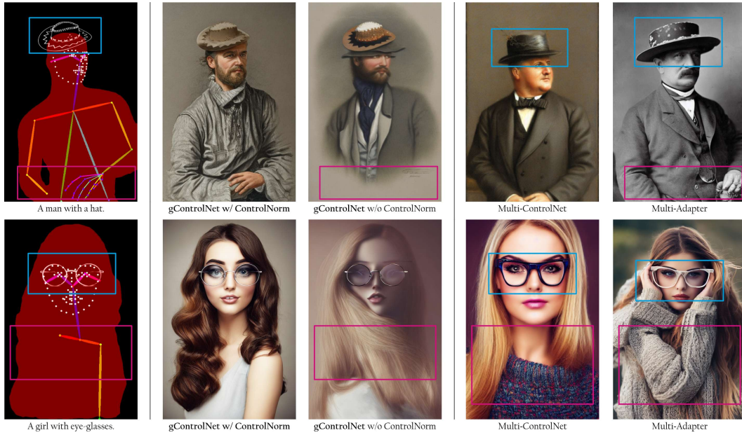
Figure 9: ControlNorm can address the imbalance among various modalities. Note that the framed areas in magenta and cyan do not provide a high-fidelity interpretation.
